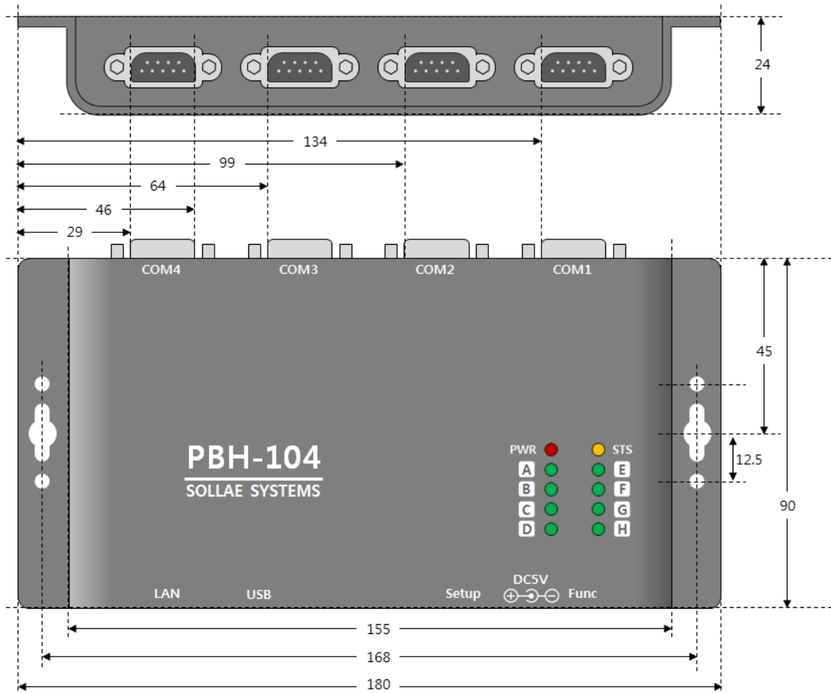
Figure 1-1 dimension
