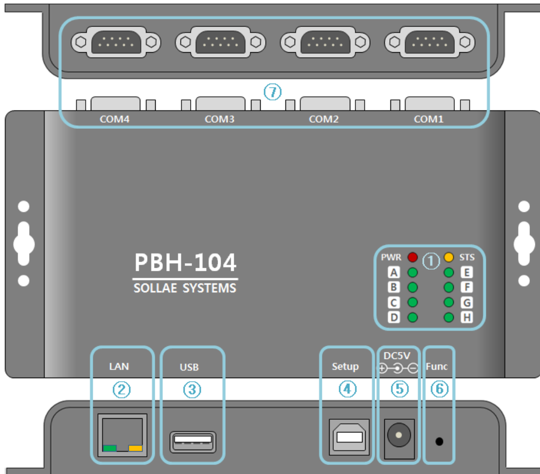
Figure 1-2 panel layout
