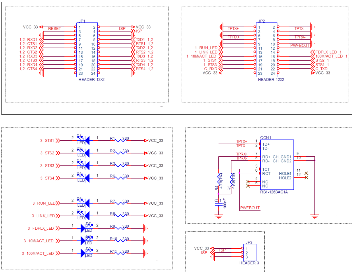
Figure 1-6 an Application Circuit
