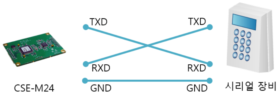
Figure 9-1 RS232 connection
